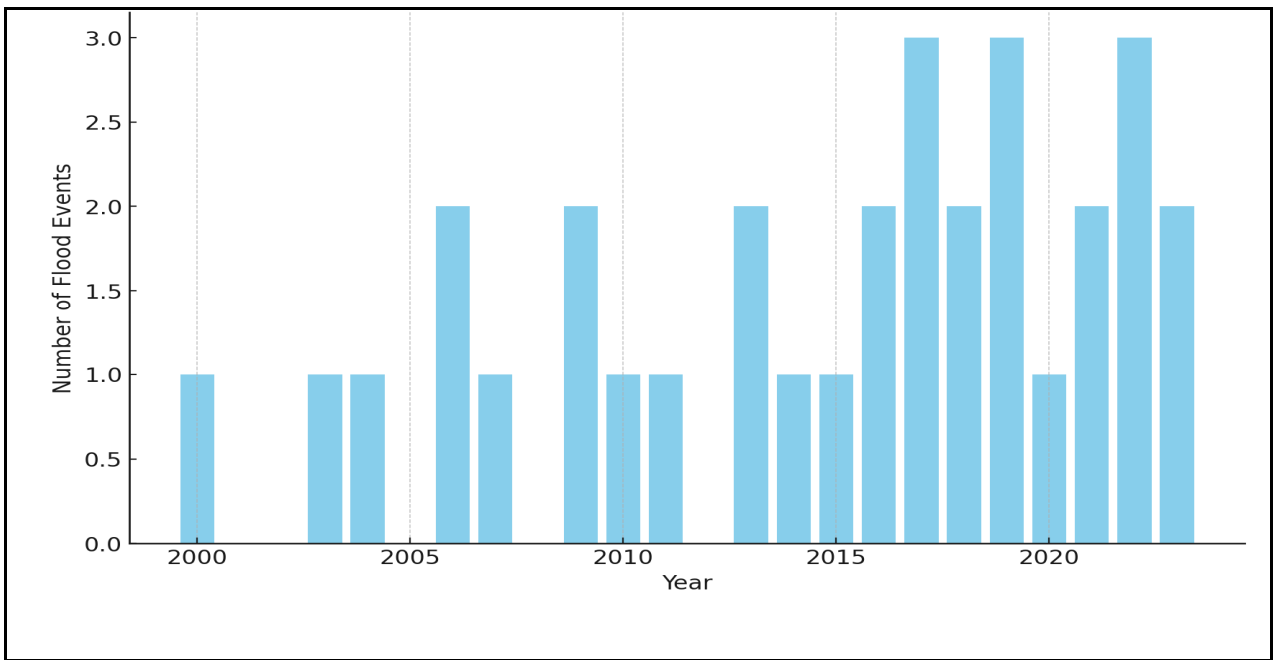
Figure 3: Recorded Flood Events in Benue River Basin (2000-2023)
